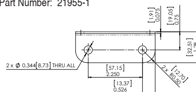
Mounting Bracket Part Number: 21955-1
