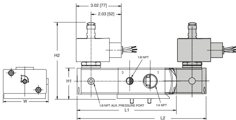
8551 NAMUR Footprint
