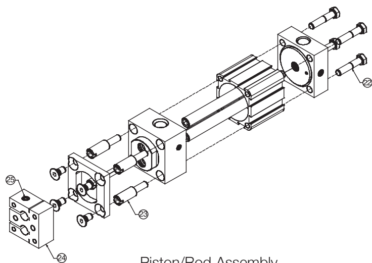
Piston/Rod Assembly
