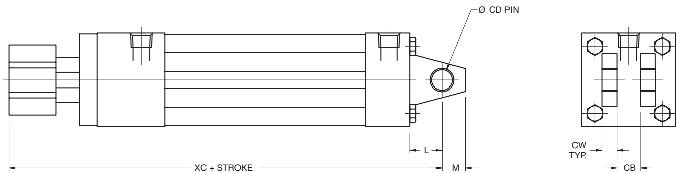
NFFPA Mount Code MP1
