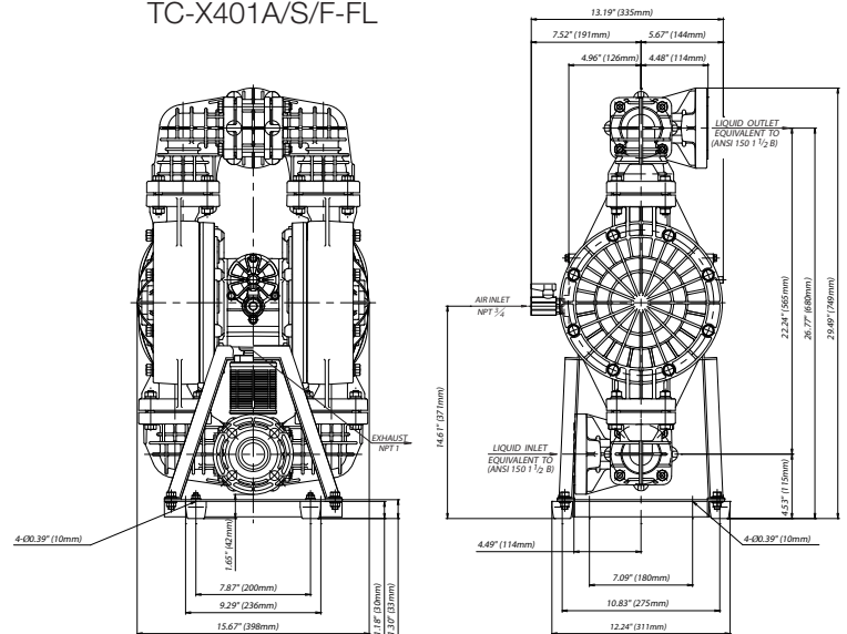
TC-X401A/S/F-FL
