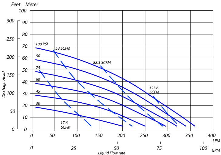
TC-X401PT VT
